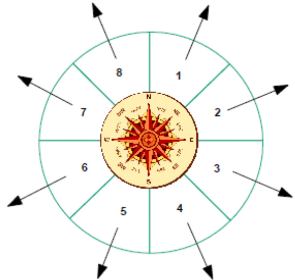
Figure 5: Directional Atlas Clusters: 8-Cluster version
