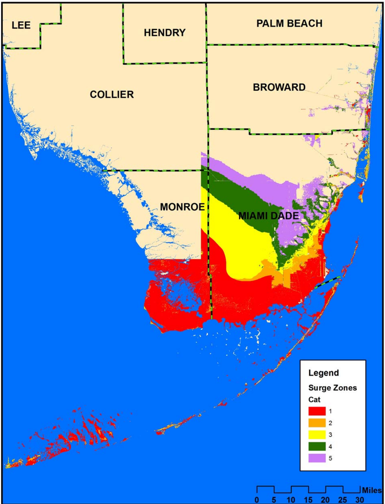
Figure 10A Directional N-NE Storm Surge for the South Florida Region
