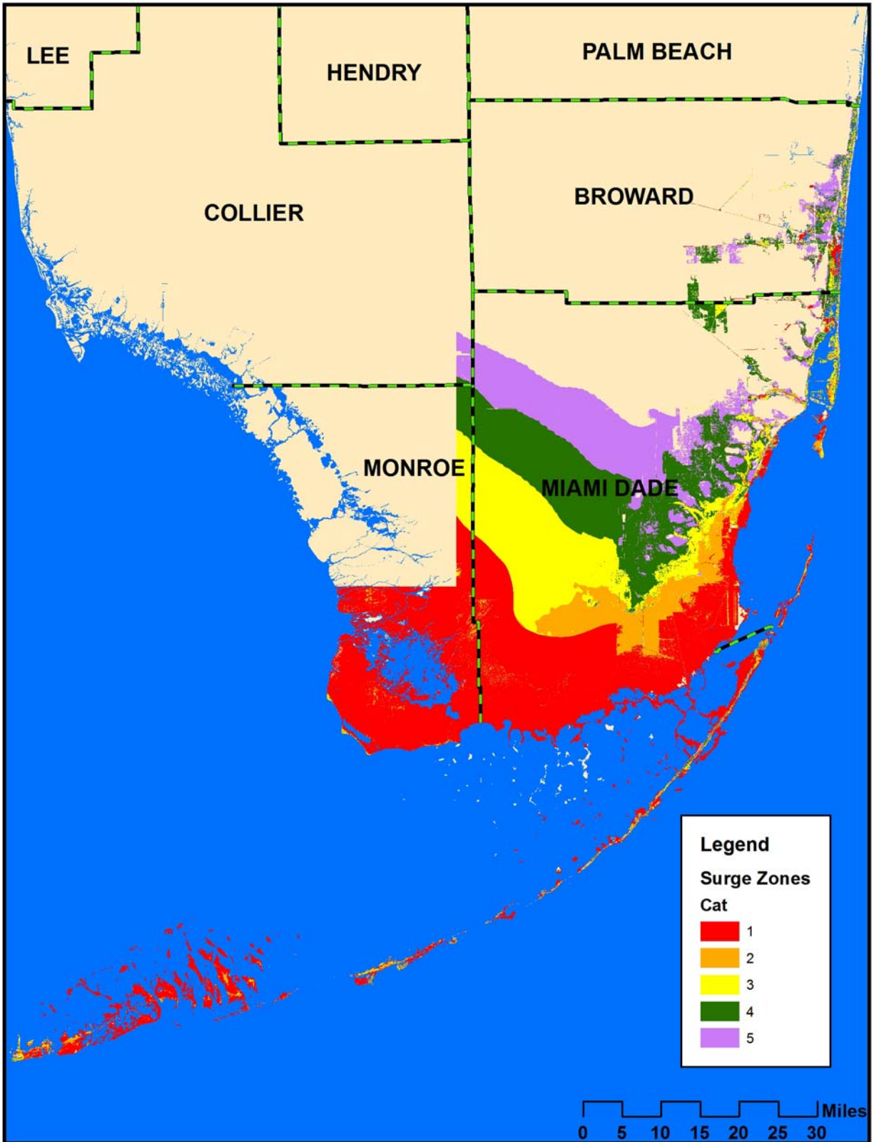
Figure 10C Directional W-NW Storm Surge for the South Florida Region
