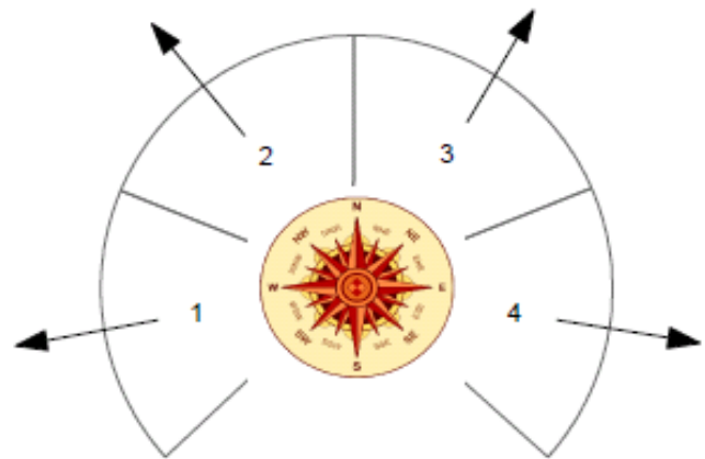
Figure 6: Directional Atlas Clusters: 4-Cluster version
