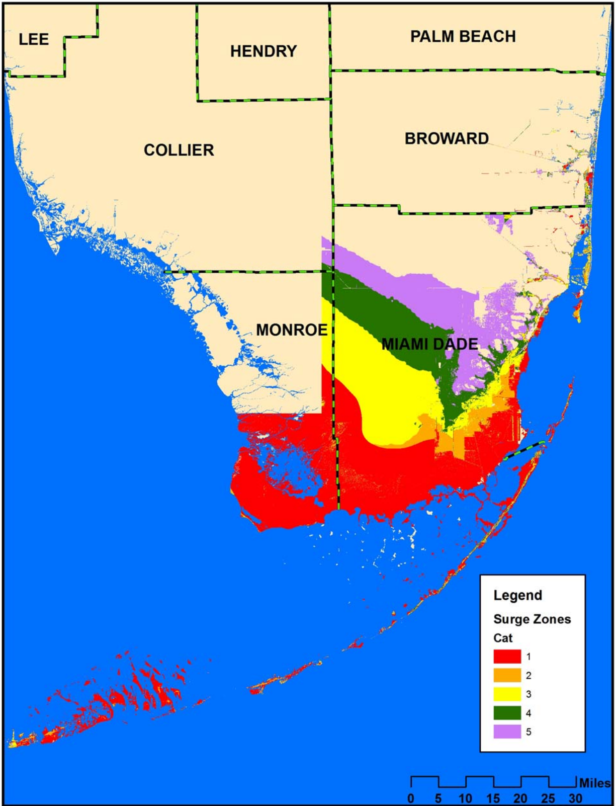
Figure 10B Directional NE-E Storm Surge for the South Florida Region
