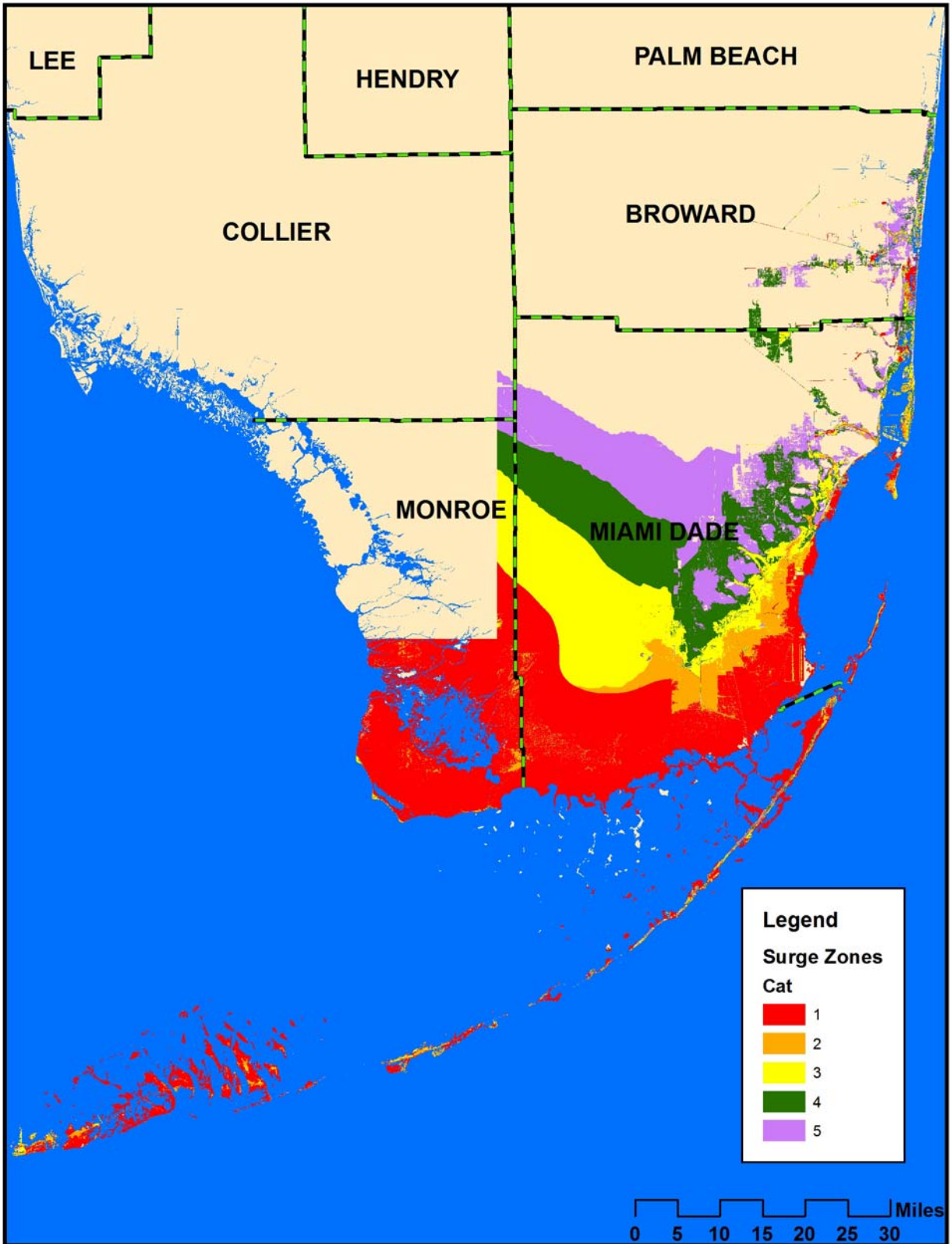
Figure 10D Directional NW-N Storm Surge for the South Florida Region
