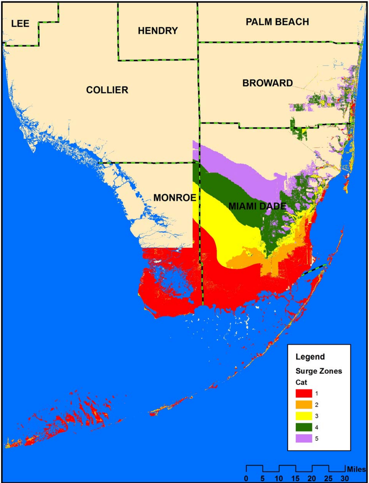
Figure 10E Directional WSW-WNW Storm Surge for the South Florida Region
