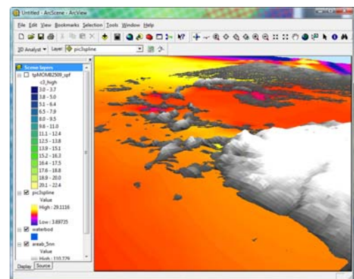
Figure 9 SLOSH Display Post-Processing
