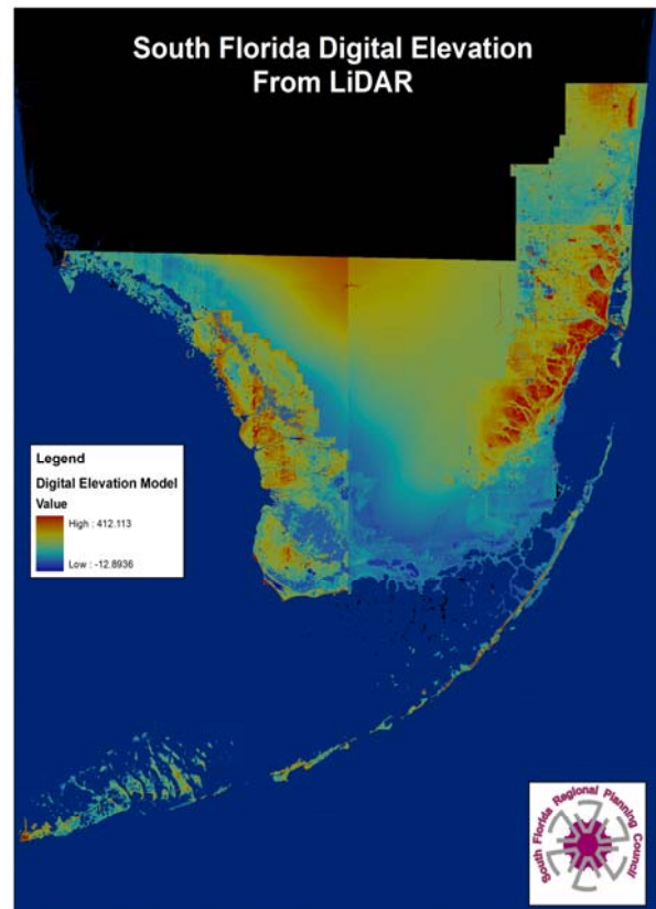
Figure 7 Digital Elevation from LIDAR
