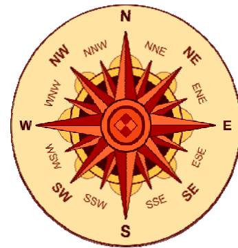
Figure 4: Compass Directions for Directional Atlas
