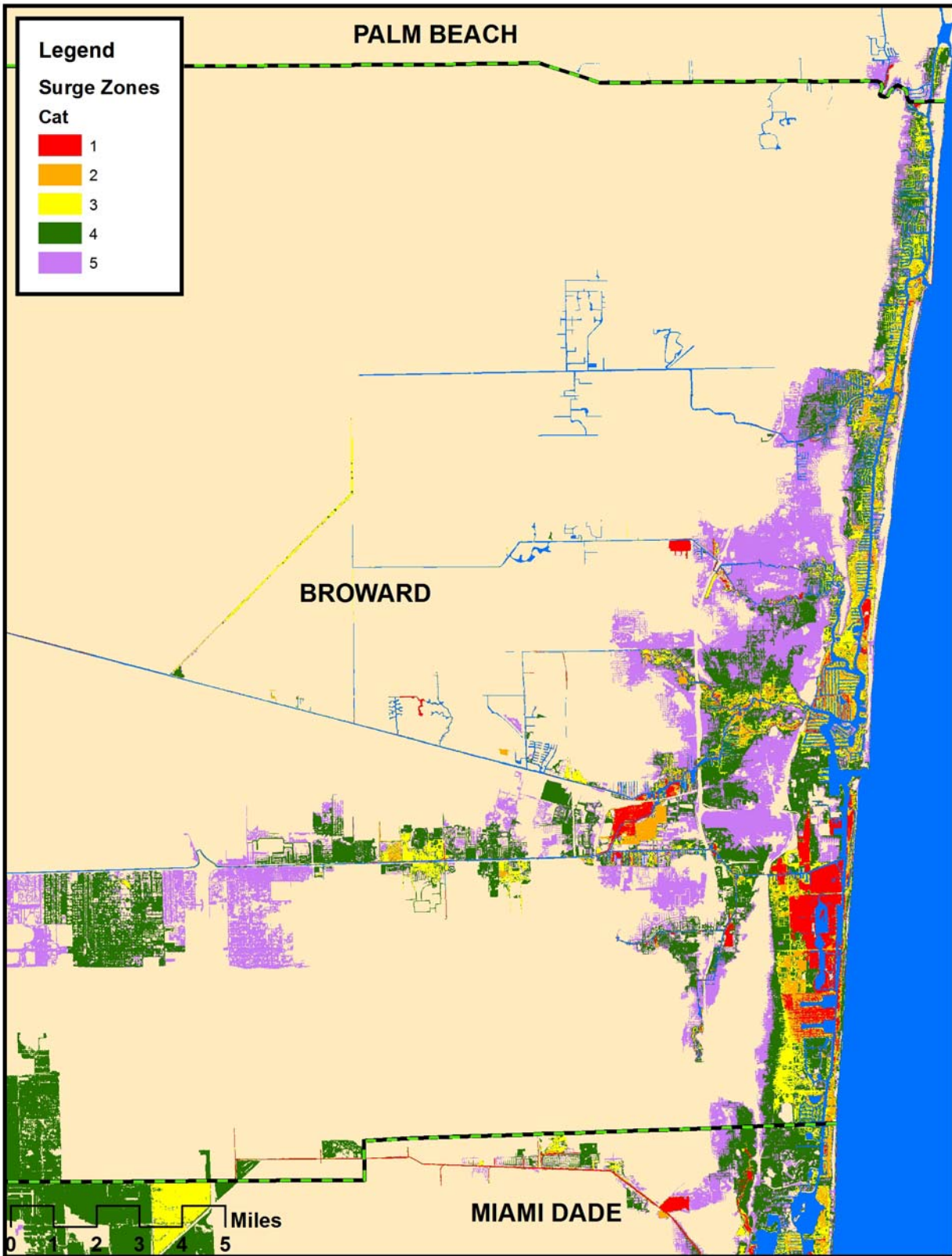
Figure 1 Directional W-NW Storm Surge for Broward County
