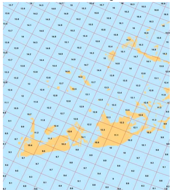
Figure II-2b: Florida Bay SLOSH Grid with surge values
