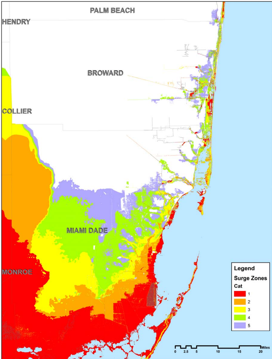
Figure II-3a South Florida Region Storm Tide Map Biscayne Bay Basin
